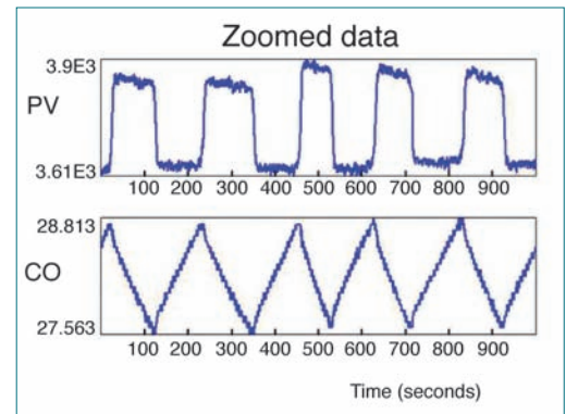
Fig. 2: Limit cycle of a process variable.
