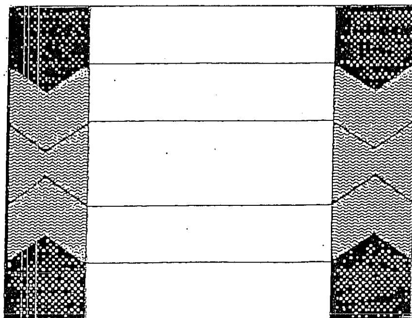
Fig. 5: Cross-section of the Walworth Style EAF 100-001 stem packing.
