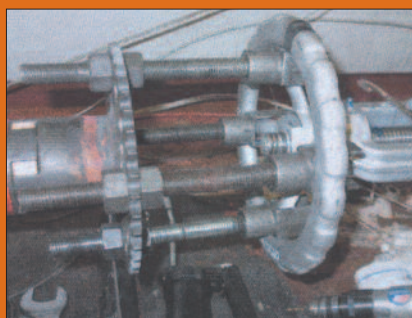
Fig. 2a: A connection from the gearmotor to the handwheel is made to minimize side-loading.
