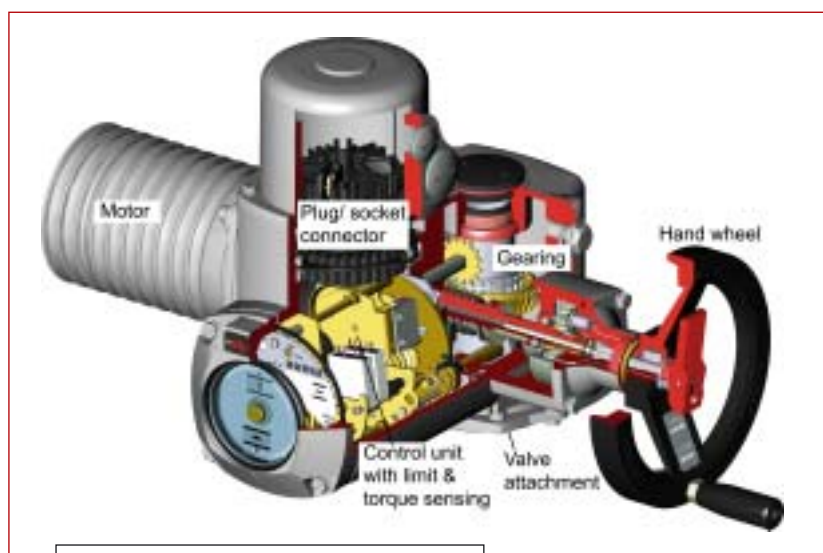
Figure 1: Typical design of an electric actuator
