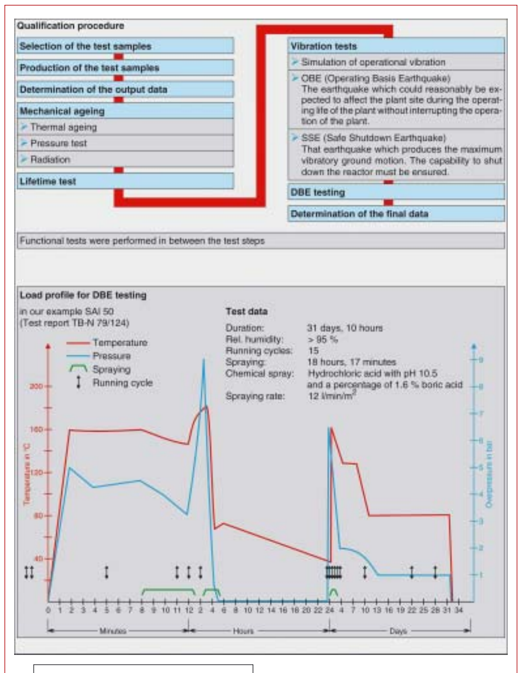
Figure 6: LOCA test for the multi-turn actuator SAI
